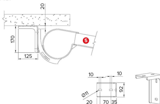
Attacco a soffitto . Ceiling application 088-920
