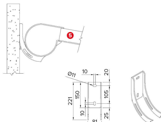
Staffa attacco parete . Wall application bracket OPTIONAL 088-902
