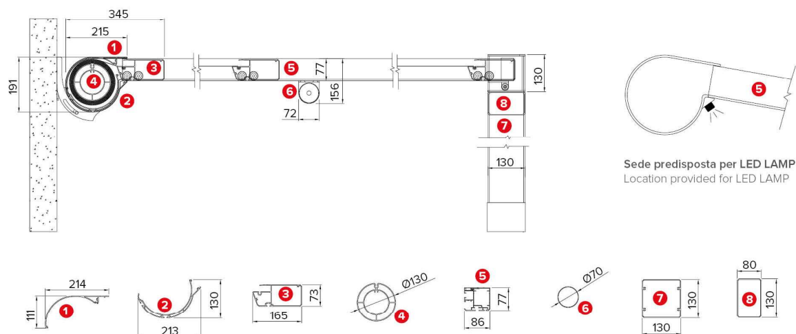
Vista frontale . Frontal view
