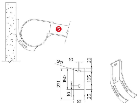
Staffa attacco parete . Wall application bracket
