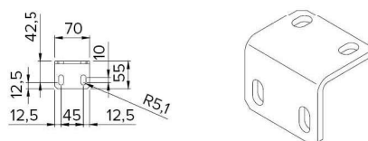
Attacco a spallina . Inside application OPTIONAL 088-914
